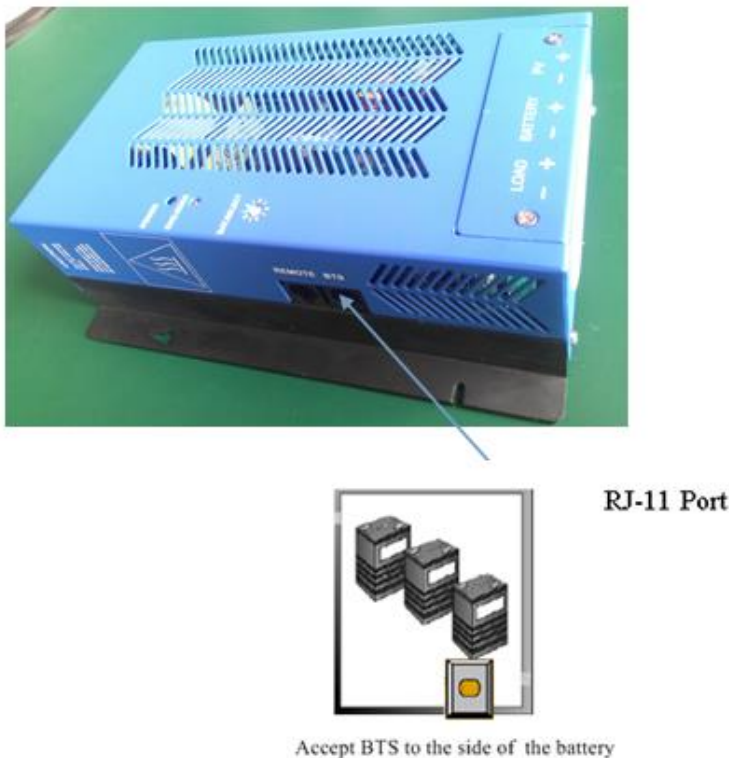
Figure 1 – 12: Install BTS
