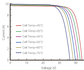
Current-Voltage Curve (LR6-60OPD-335M)
